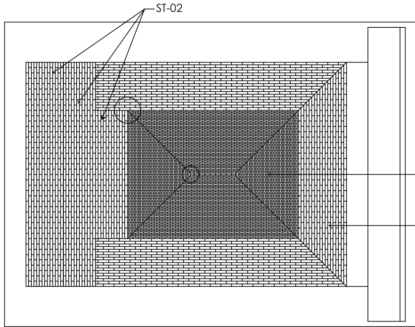
SPA TILE PLAN VIEW
