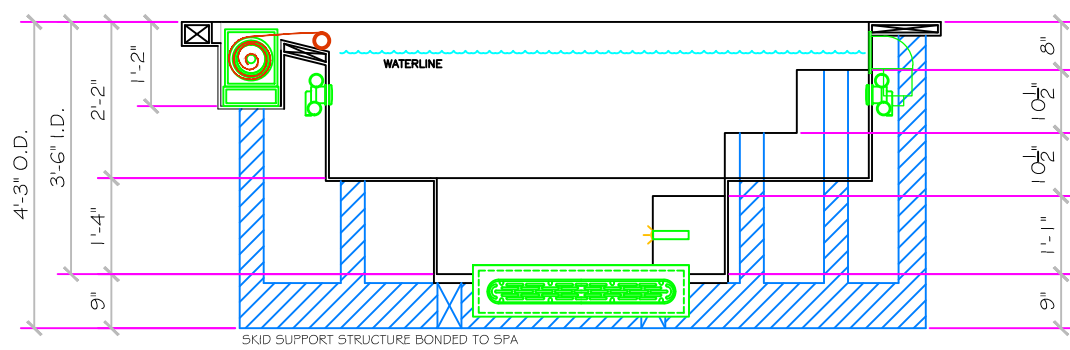
SECTION B-B
