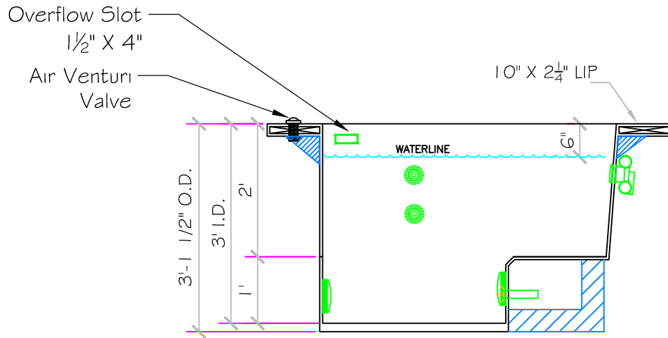
WEST SECTION
