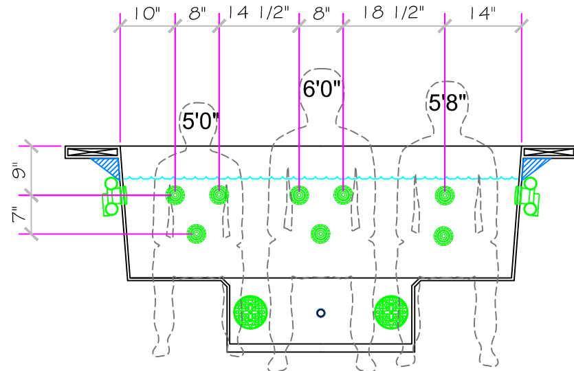
NORTH SECTION
