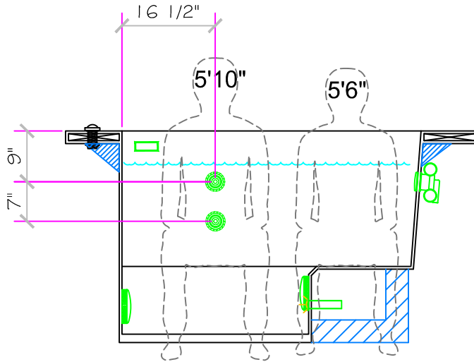
WEST SECTION
